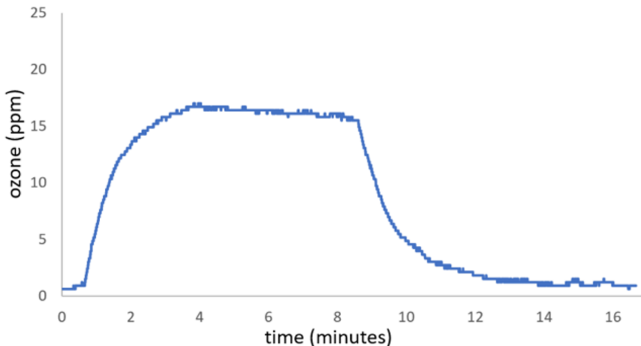
Figure 5. This is the same setup as the two figures immediately above, but in this case the lid of the box was opened only slightly, enough to allow a 3/16" ID thick-wall silicone tube to be introduced, through which ozone was pumped into the box. The ozone generator was able to exceed the minimum desired concentration of 10 ppm, but only achieved about 17 ppm, and was unable to easily achieve 20 ppm as it had when the lid was tightly and correctly fitted. LESSON: you can just flop the ozone tube into the box if you don't have a drill, but it will not work as well. Note also that, unlike the first figure above, the ozone concentration decay is very rapid even when the lid is only cracked open slightly.
