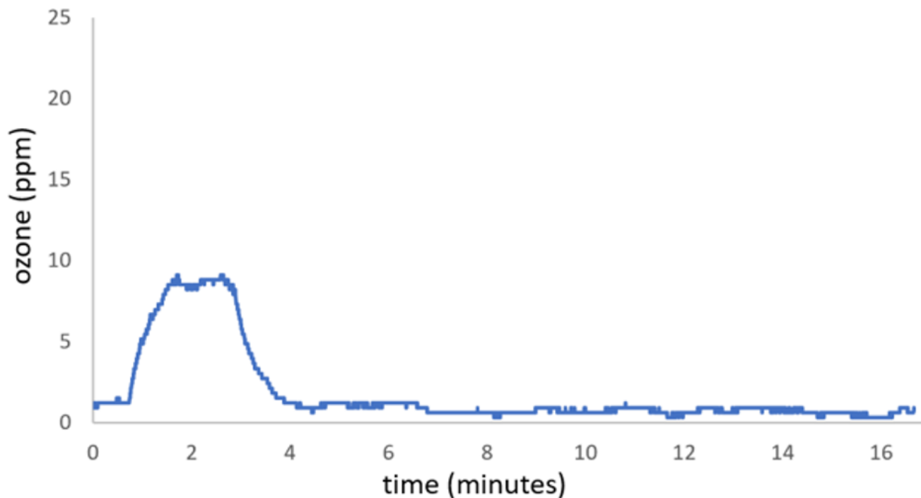
Figure 4. The same setup as the figure immediately above, but with the lid loosened and slid to the side slightly to allow a 1 cm gap on one side, allowing ozone to easily diffuse from the box. With such a large leak, we were unable to achieve the minimum desired ozone concentration of 10 ppm. The generator was able to maintain a concentration of approximately 9 ppm if left ON, but when switched OFF, the ozone concentration in the box quickly decayed to baseline. LESSON: lids should fit tightly and be placed properly.
