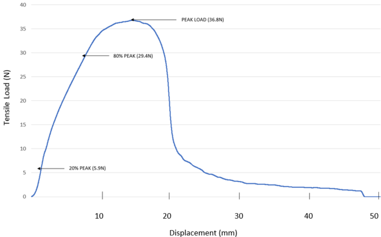
Figure 8. Indication of the key points for calculations on each tensile data chart: peak load, 80% peak load, and 20% peak load. Toughness energy calculations represent a calculation under the curve from zero to the indicated point (20% or peak) in units of mJ.
