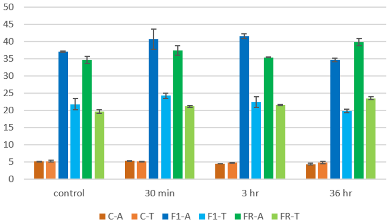
Figure 9. Peak Load (N) for each of the materials tested, along (“A”) and transverse (“T”) to the rolling direction during fabrication. Ozone exposure times were zero (control), 30 minutes, 3 hours, and 36 hours. For any given material and test axis orientation, no effect of ozone exposure was evident up to 36 hours at 20 ppm (equivalent to 72 half-hour (30-minute) disinfection cycles).
