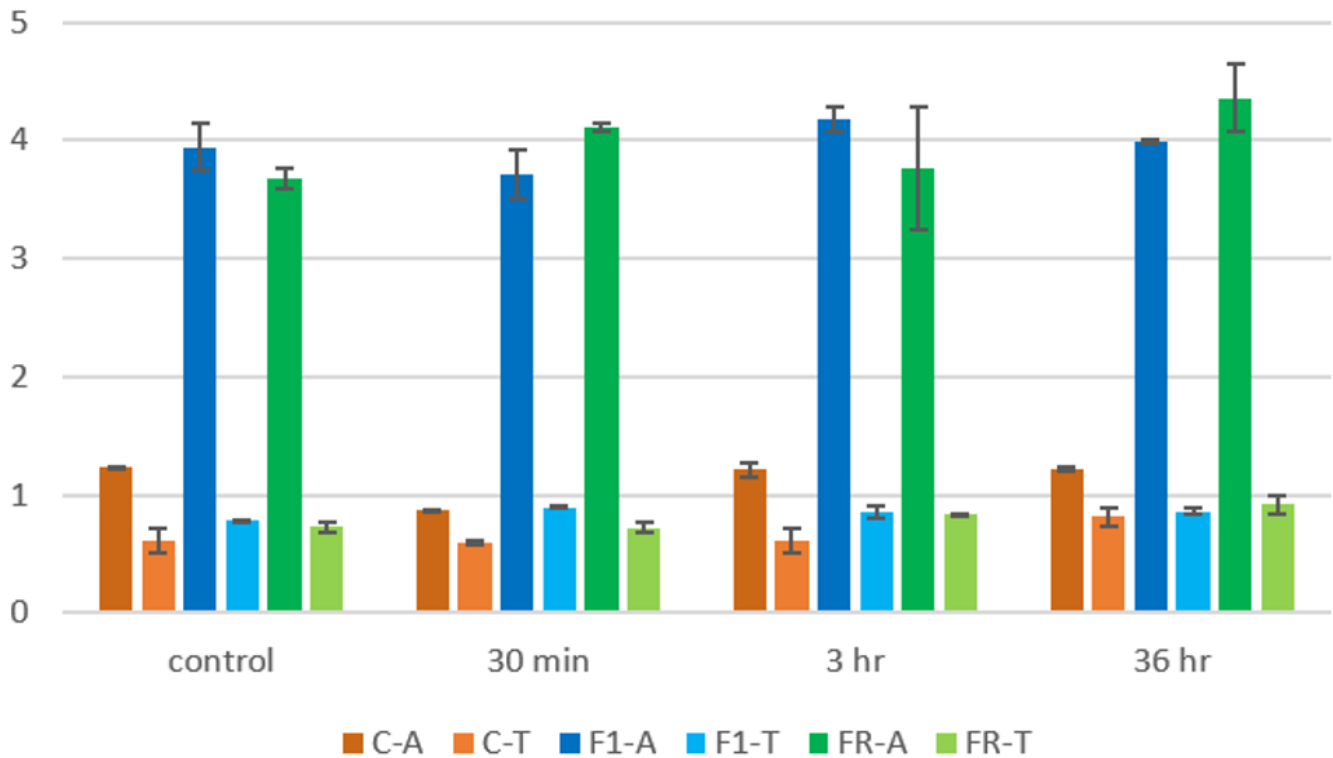
Figure 12. Stiffness (N/mm of gage length elongation) from 20% to 80% peak load for each of the materials tested, along and transverse to the rolling direction during fabrication. Ozone exposure times were zero (control), 30 minutes, 3 hours, and 36 hours. For any given material and test axis orientation, no effect of ozone exposure was evident up to 36 hours at 20 ppm (equivalent to 72 half-hour disinfection cycles).
