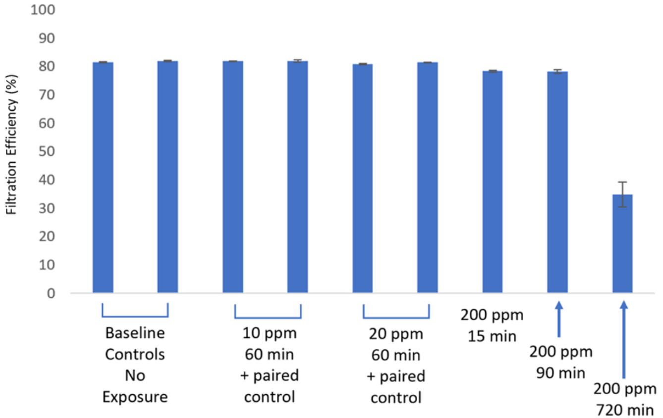
Figure 2. Filtration efficiency of uncharged MSP. The first six bars (to the left) each represent seven samples, whereas the three bars to the right, for the highest ozone dosages, represent 5 samples each. Filtration efficiency was not detectably changed when comparing control fabric samples to those exposed to 10ppm or 20ppm ozone, always achieving a filtration efficiency of 81% to 82%. A small but detectable drop in filtration efficiency was indicated at 200 ppm for 15 minutes and 90 minutes (filtration efficiency dropped to 78.4% and 78.2%, respectively). This is a small reduction in filtration efficiency, corresponding to an ozone disinfectant dosage of 18,000 ppm-minutes. Only at the most extreme ozone dosage, 200 ppm for 720 minutes, is a major reduction in filtration efficiency observed, down to 34.9%, at an ozone dose of 144,000 ppm-minutes. Mean and standard error bars are shown.
