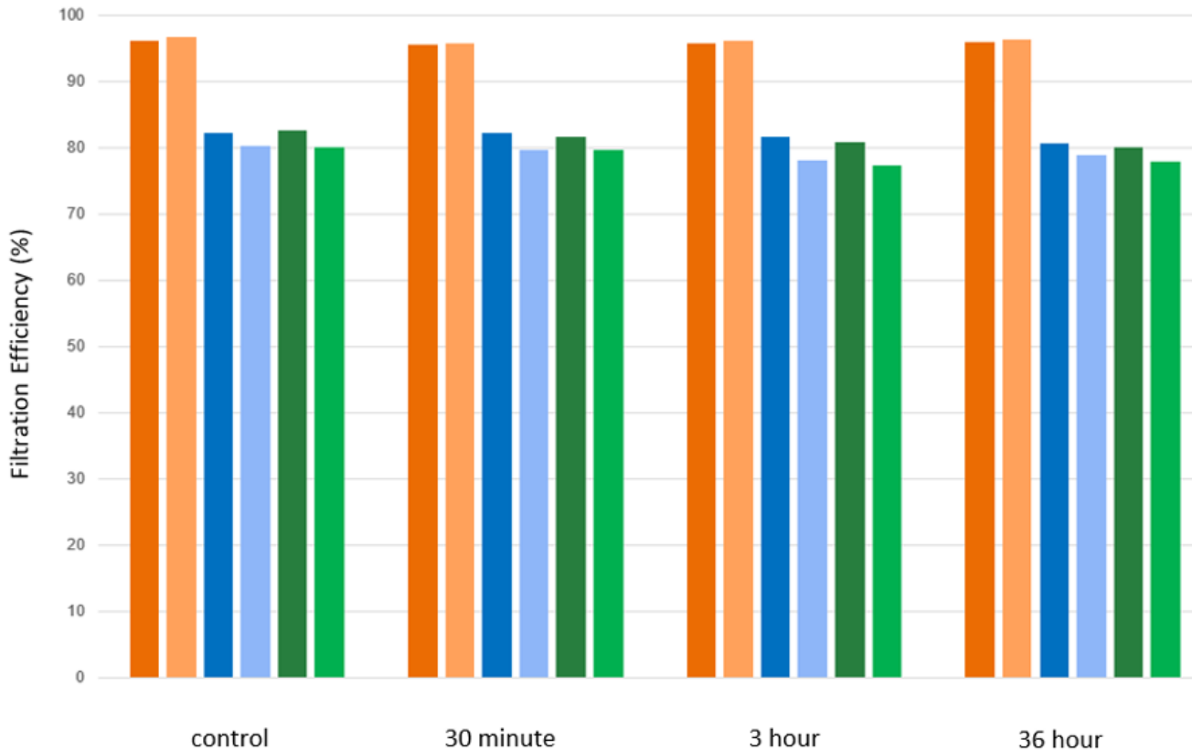
Figure 5. Effect of ozone exposure on charged classical N95 MBM and novel MSP. Orange bars show the effect of ozone on the filtration efficiency of the classical N95 material. Dark orange is tested after ozone exposure without any re-charging afterward, light orange shows the results of the material being recharged after ozone exposure. Blue and green bars show the effect of ozone exposure on triboelectrically-charged (F1) MSP filter material, dark blue is before corona recharge following ozone exposure, light blue is after ozone exposure then corona recharge. Similarly, green bars show the effects on FR material.
