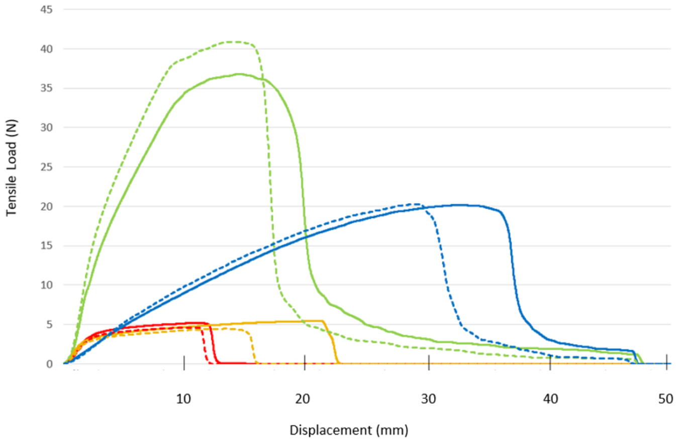
Figure 6. Typical load-deformation curves for the filter material, showing the strong anisotropic behavior of these materials. Red and yellow lines represent classical N95 MBM. Red is along the roll direction, yellow is transverse. Green and blue lines are MSP material. Green lines are along the roll direction, blue is transverse. Solid lines represent materials before ozone exposure, dashed lines represent properties after ozone exposure (20 ppm for 36 hours).
