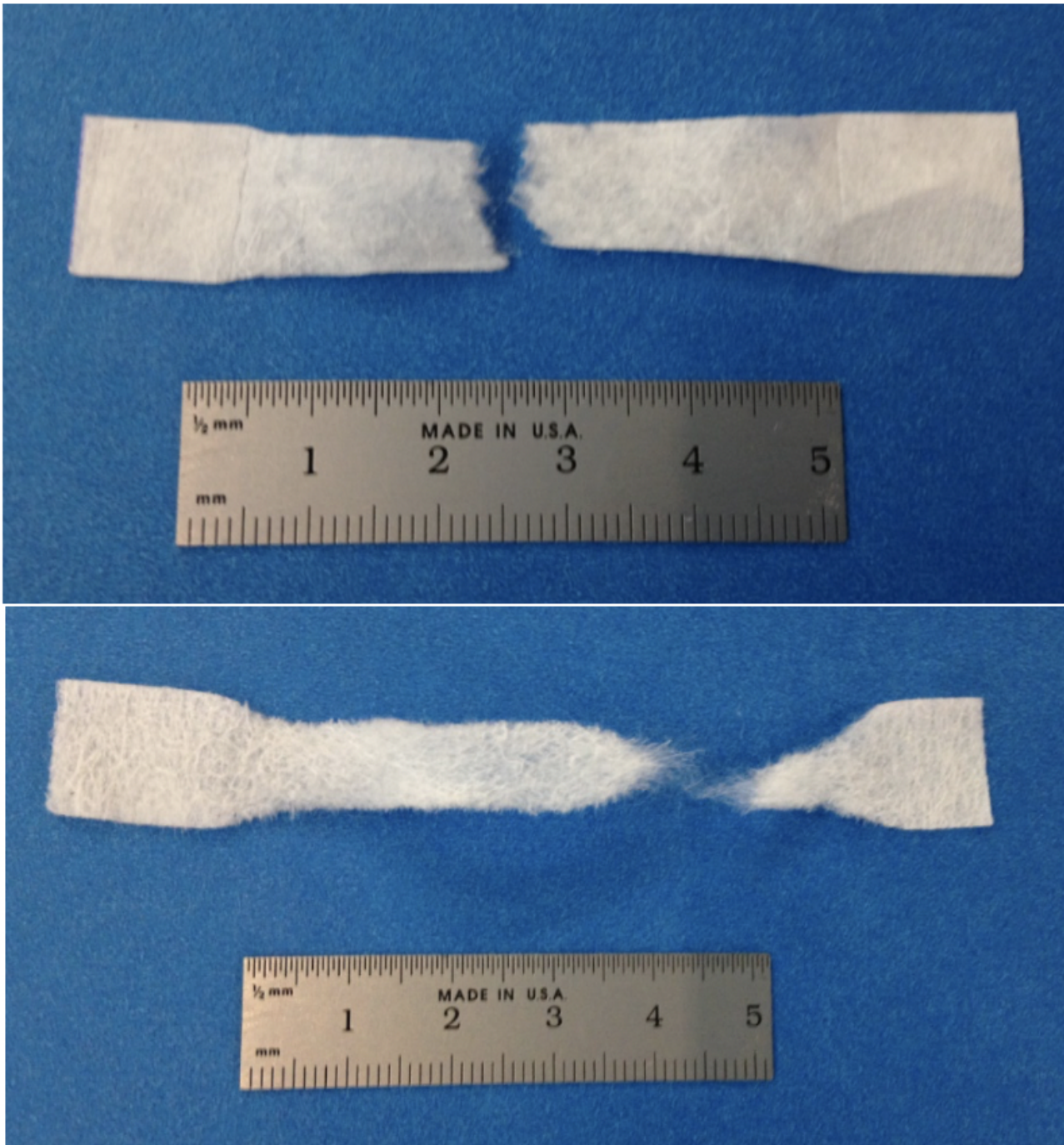
Figure 7. Typical tensile specimens after loading to failure. The classical N95 mask (MBM) filter fabric (above) failed at much lower load and elongation than the MSP filter material (below)
