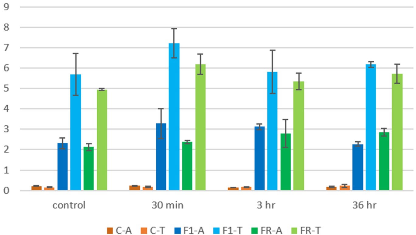
Figure 11. Strain energy (mJ) from zero to 20% peak load for each of the materials tested, along and transverse to the rolling direction during fabrication. Ozone exposure times were zero (control), 30 minutes, 3 hours, and 36 hours. For any given material and test axis orientation, no effect of ozone exposure was evident up to 36 hours at 20 ppm (equivalent to 72 half-hour disinfection cycles).
