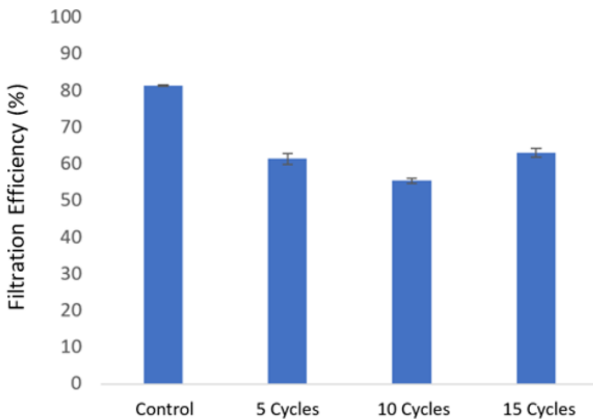
Figure 3. Filtration efficiency of the novel MSP material after laundering.
