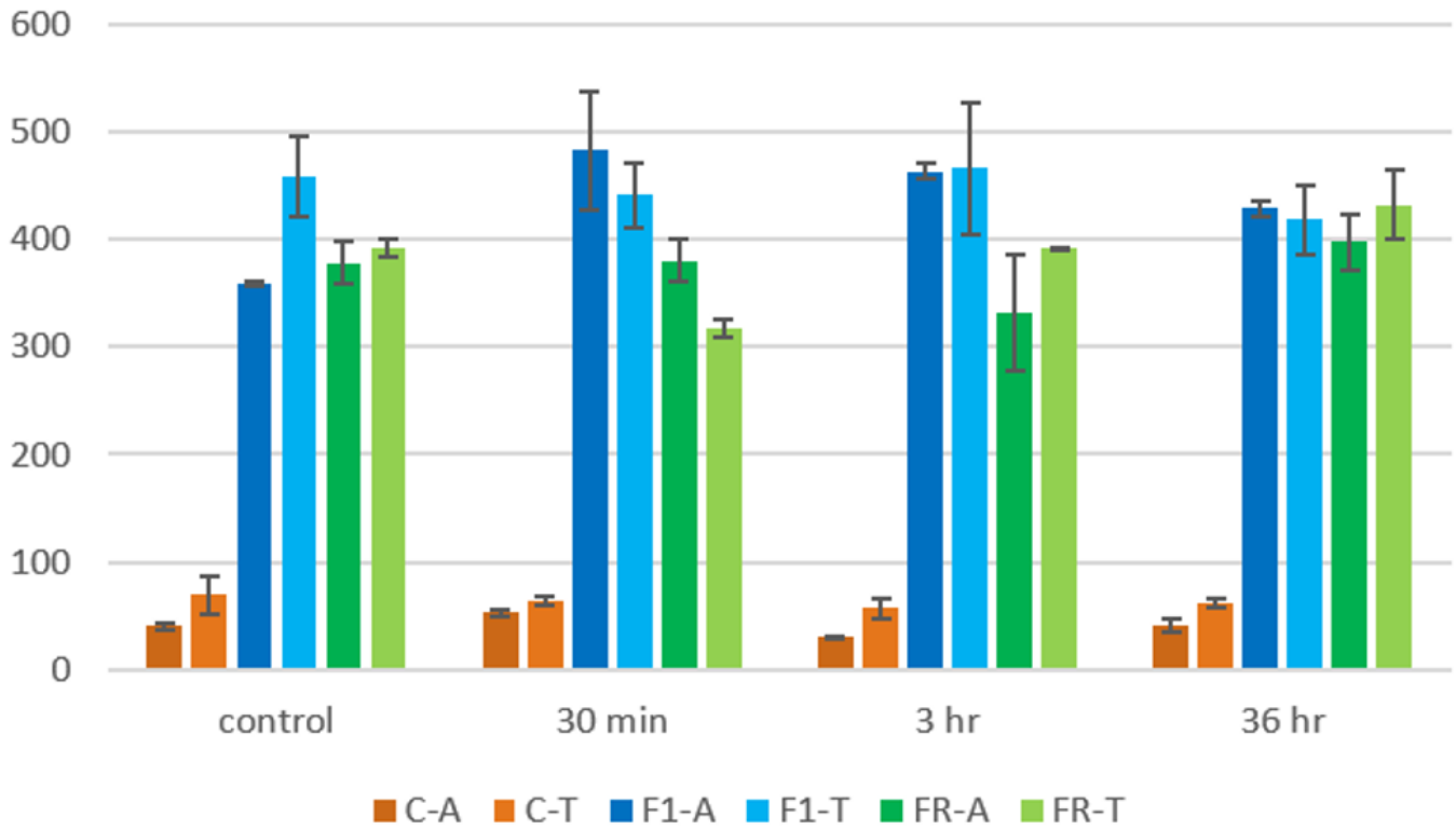
Figure 10. Strain energy (mJ) from zero to peak load for each of the materials tested, along and transverse to the rolling direction during fabrication. Ozone exposure times were zero (control), 30 minutes, 3 hours, and 36 hours. The number of data samples was small, but no trend suggesting a degradation of performance is evident. For any given material and test axis orientation, no effect of ozone exposure was evident up to 36 hours at 20 ppm (equivalent to 72 half-hour disinfection cycles).
