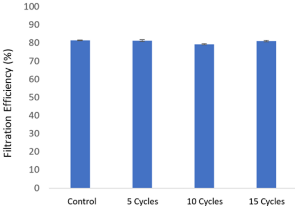
Figure 4. Filtration efficiency of MSP material after laundering followed by electrostatic charging.
